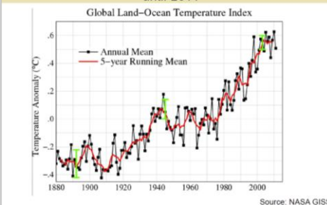
Warming has not « stopped »: Global (land & ocean) mean surface temperature change from NASA GISS until 2011
